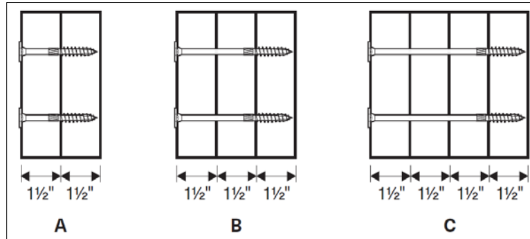
Figure 9. Big Timber Screw Sawn Lumber Assemblies
