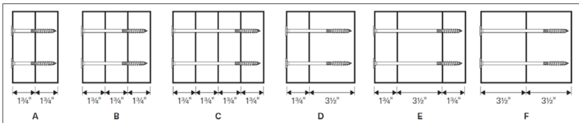
Figure 10. Big Timber Screw SCL Assemblies
